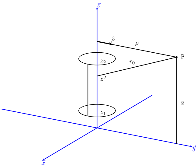
Figure 4. Current-Filament Geometry for the Thin-Wire Kernel.
