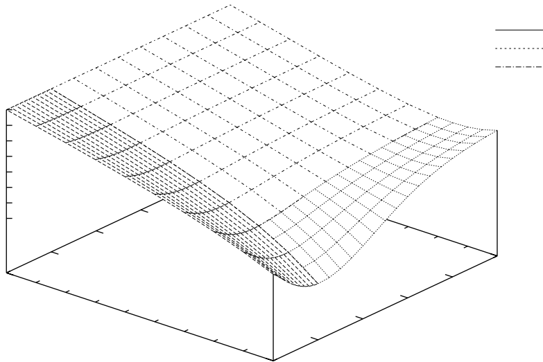
Figure 7(b). \text{Im}(I_\rho^V) for \epsilon_1/\epsilon_0=4 , \sigma_1=0.001 mhos/m, frequency = 10 MHz.
