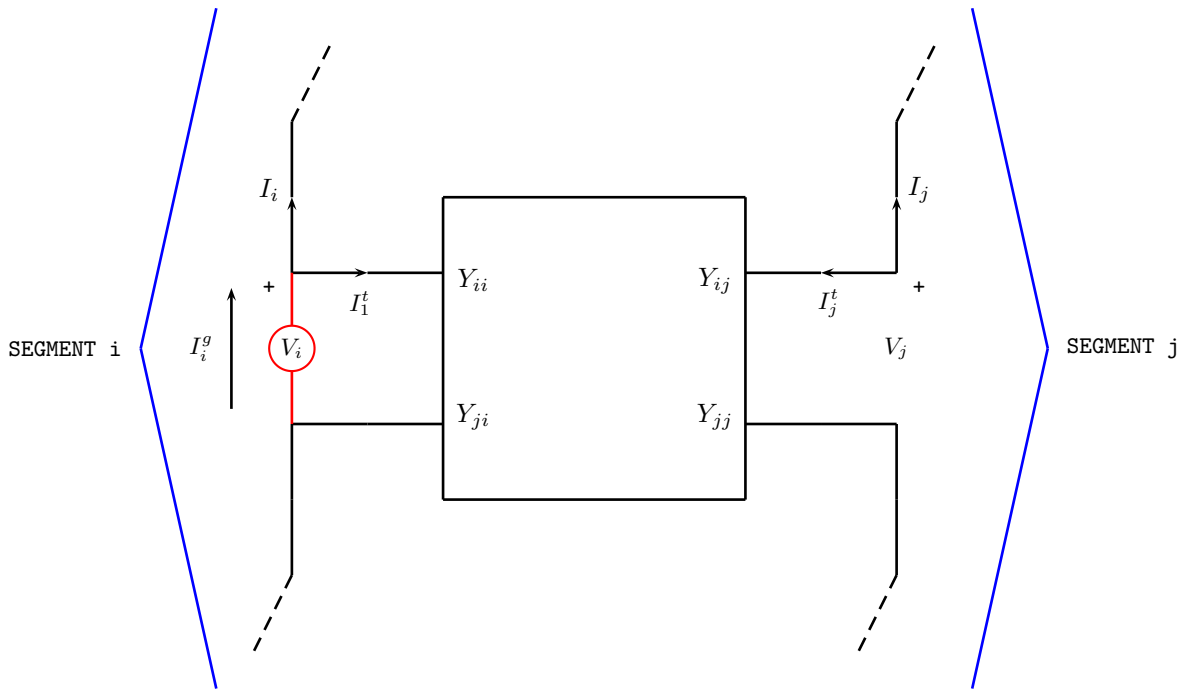
Figure 21. Network Port and Voltage Source Connected to a Segment.
