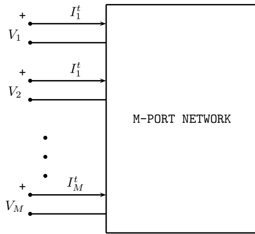
Figure 19. Voltage and Current Reference Directions at Network Ports.
