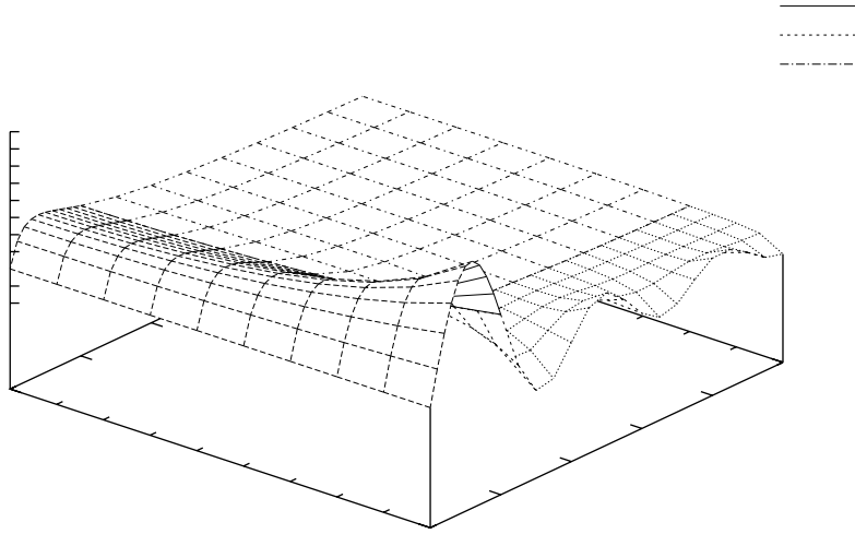
Figure 11(a). \text{Re}(I_\rho^H) for \epsilon_1/\epsilon_0=16 , \sigma_1=0.000 mhos/m, frequency = 10 MHz.
