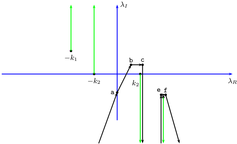
Figure 15. Contour for Evaluation of Hankel Function Form of Sommerfeld Integrals when Real Part k_1 is Large and Imaginary k_1 is Small.
