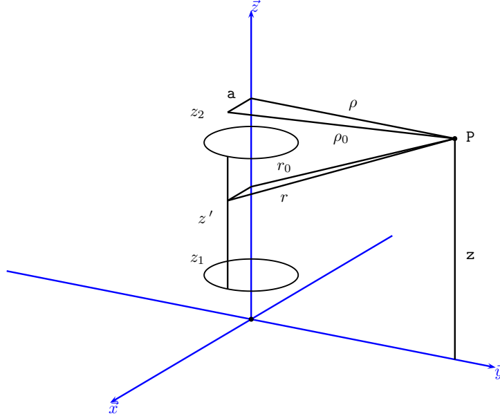
Figure 5. Current geometry for the extended thin-wire kernel.
