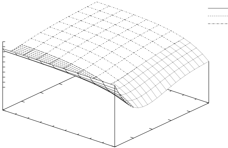
Figure 8(a). \text{Re}(I_z^V) for \epsilon_1/\epsilon_0=4 , \sigma_1=0.001 mhos/m, frequency = 10 MHz.
