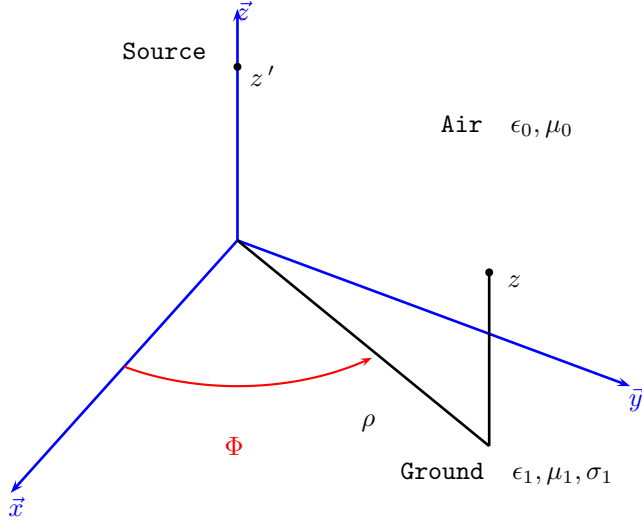
Figure 6. Coordinates for Evaluating the Field of a Current Element Over Ground.
