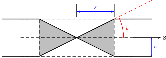
Figure 17. Biconical Transmission Line Model of Source Region.
