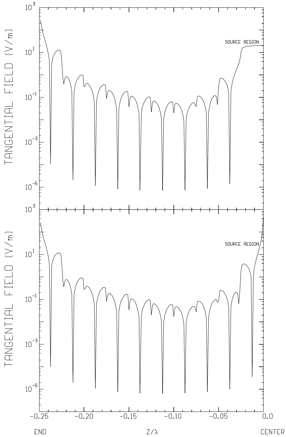
Figure 18. Field Plot for a Linear Dipole. \Omega=15 .
