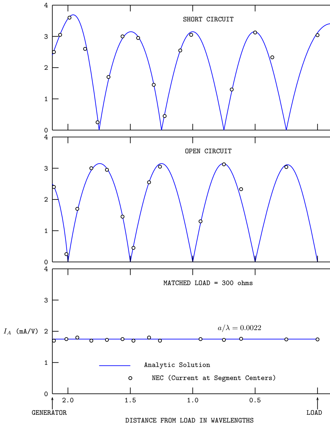
Figure 22. Current Distribution on a Two-Wire Transmission Line
