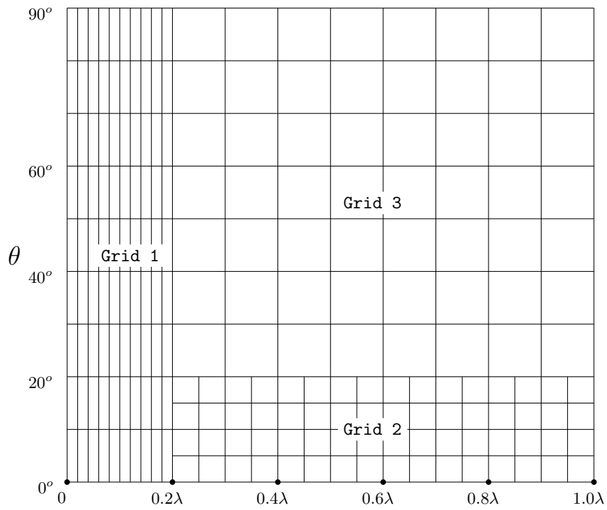
Figure 12. Grid for Bivariate Interpolation of I 's.
