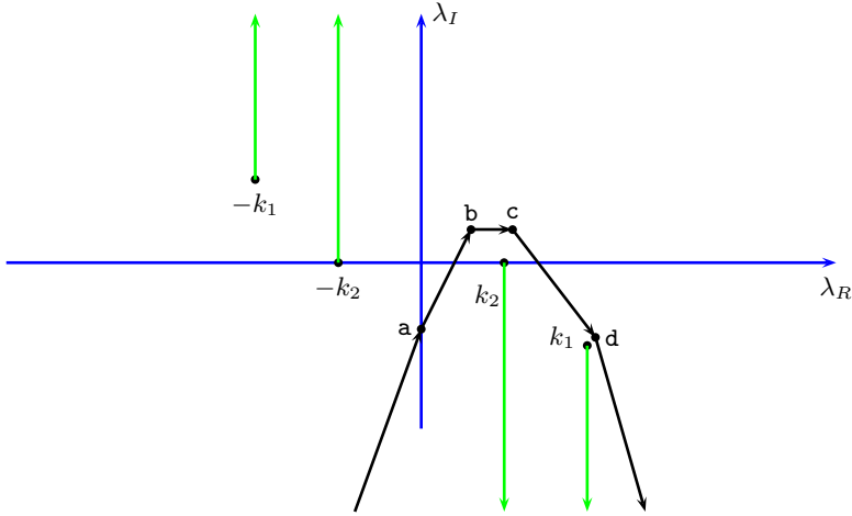
Figure 14. Contour for Evaluation of Hankel Function Form of Sommerfeld Integrals.
