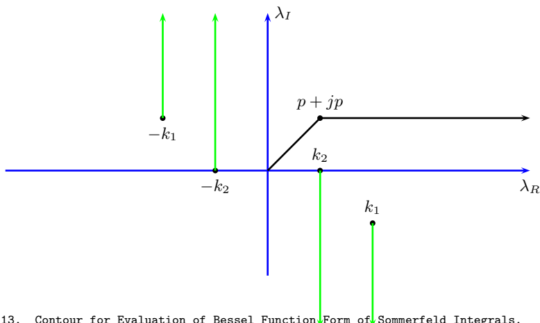
Figure 13. Contour for Evaluation of Bessel Function Form of Sommerfeld Integrals.
