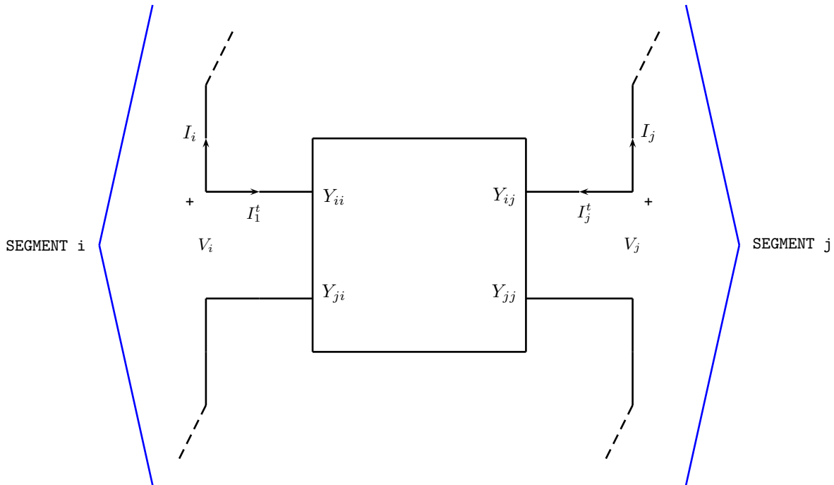
Figure 20. Network Connection to Segments.
